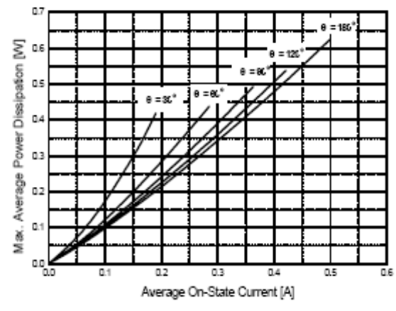
Fig 8. Power Dissipation
