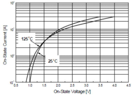
Fig.2 On-State Voltage
