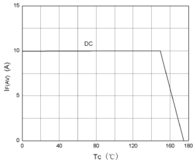
Fig. 3 Average Current versus ambient temperature (d=0.5)(per diode)
